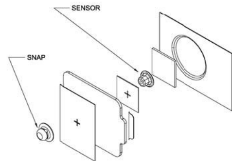
Figure 1: Schematic of Integrated ECG Electrode
